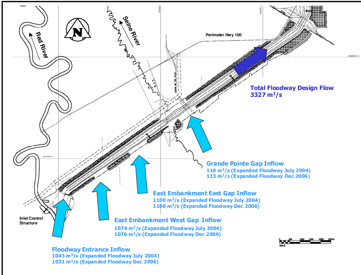
Figure 4.3-2 (b) Flow Through Floodway Embankment Gaps for Design Flow 300 Year Flood
