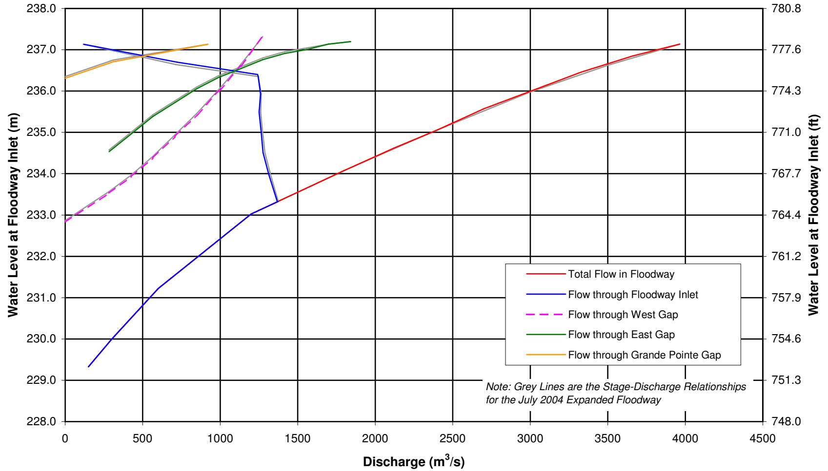
Figure 4.3-3 Flow Distribution Through Floodway Embankment Gaps
