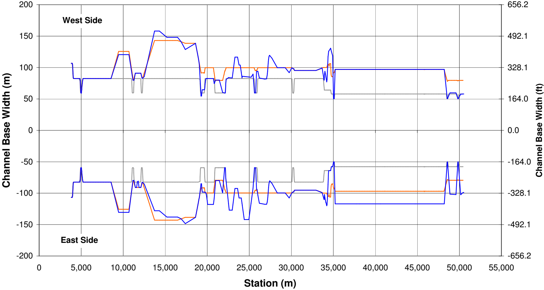
Figure 4.3-4 Floodway Channel Base Widths
