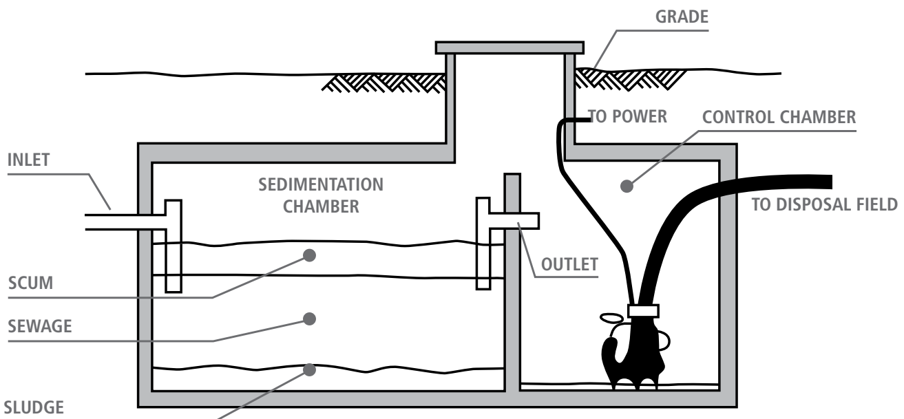
FIGURE 1 SEPTIC TANK
